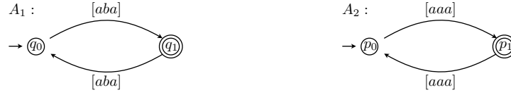
Fig. 7. Two DWA. While L(A_1) can be defined in \text{FO}(\sim, <) , L(A_2) can not.
